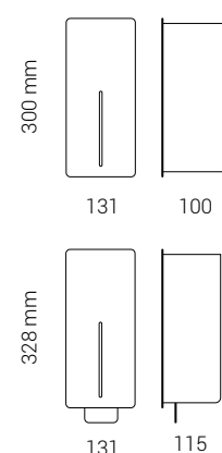
LOKI SOAP/DISINFECTANT DISPENSER
